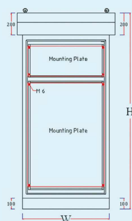
MOUNTING PLATE VIEW
